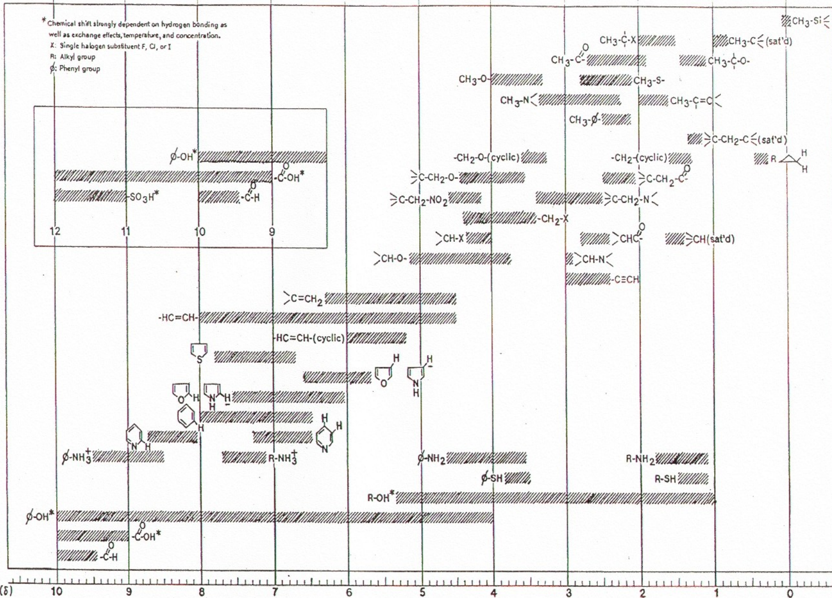
EM-360 Functional Group Correlation Chart Proton NMR Chemical Shifts
